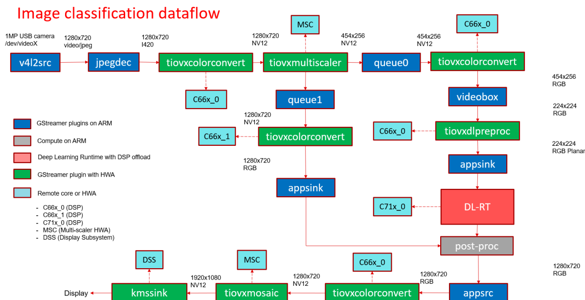
Fig. 5.6: GStreamer based data-flow pipeline for image classification demo with USB camera and display
