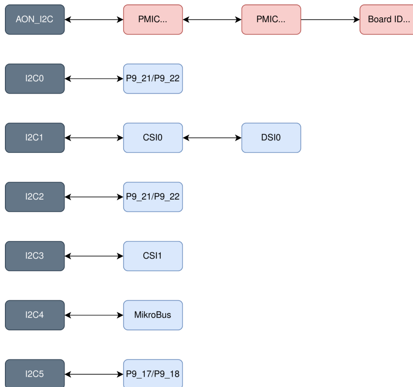
Fig. 3.2: I2C-Usage diagram
