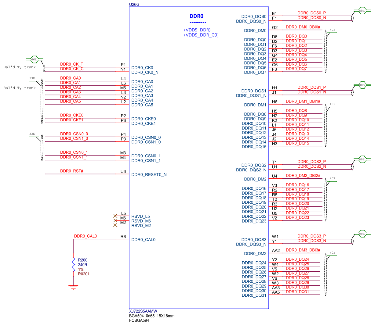
Fig. 3.17: BeagleY-AI SoC DDR0 connections
