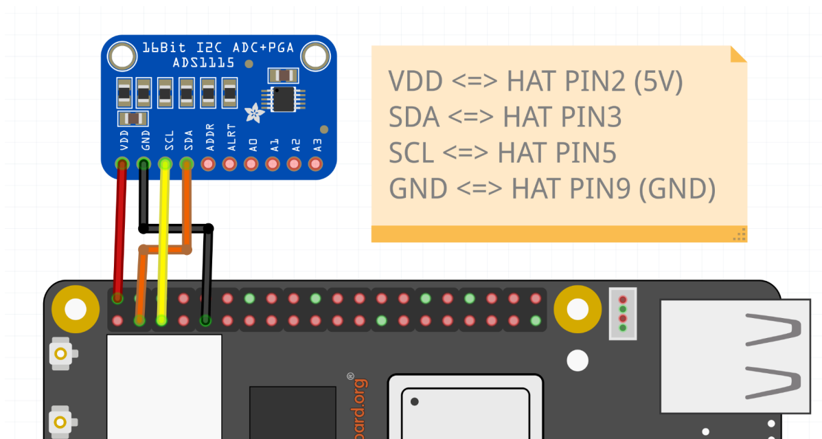
Fig. 5.26: ADS1115 connection
