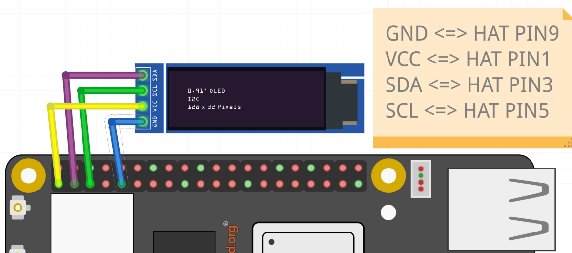
Fig. 5.16: OLED display 128x32
