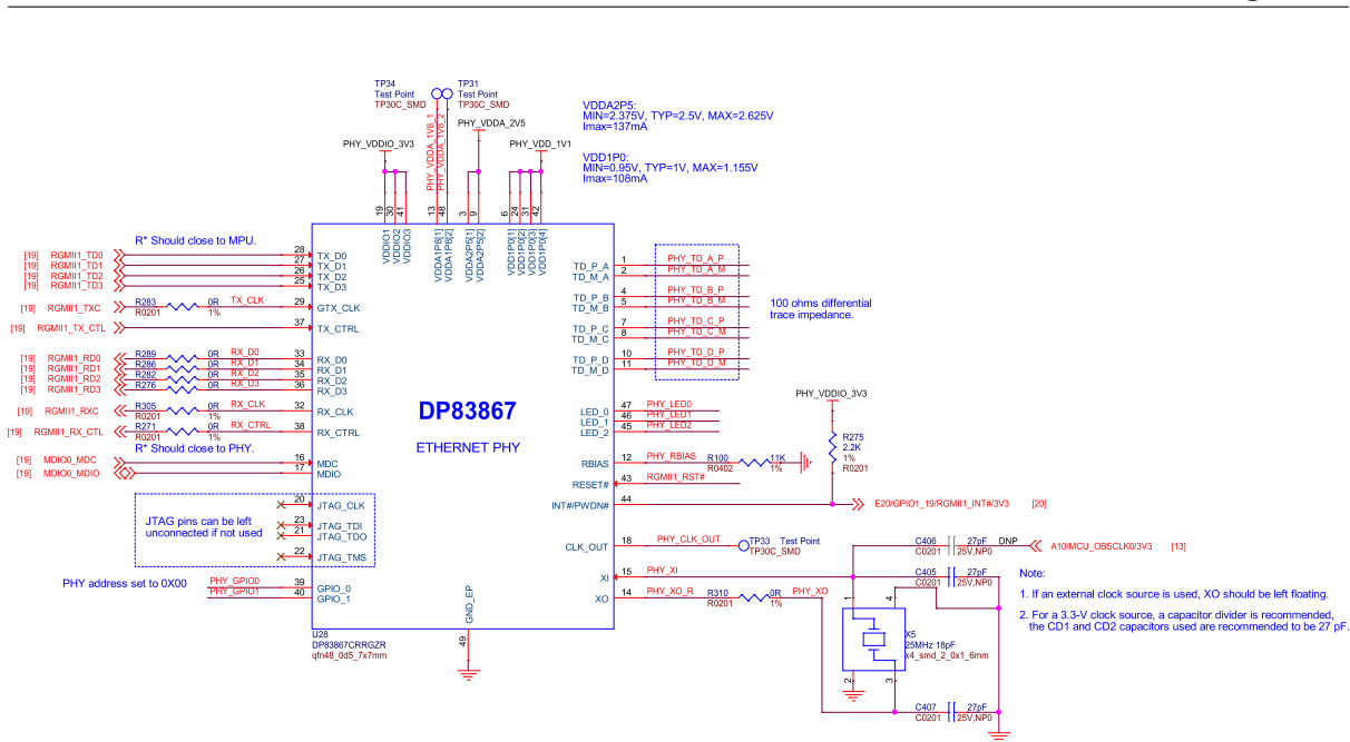
Fig. 3.39: BeagleY-AI ethernet DP83867
